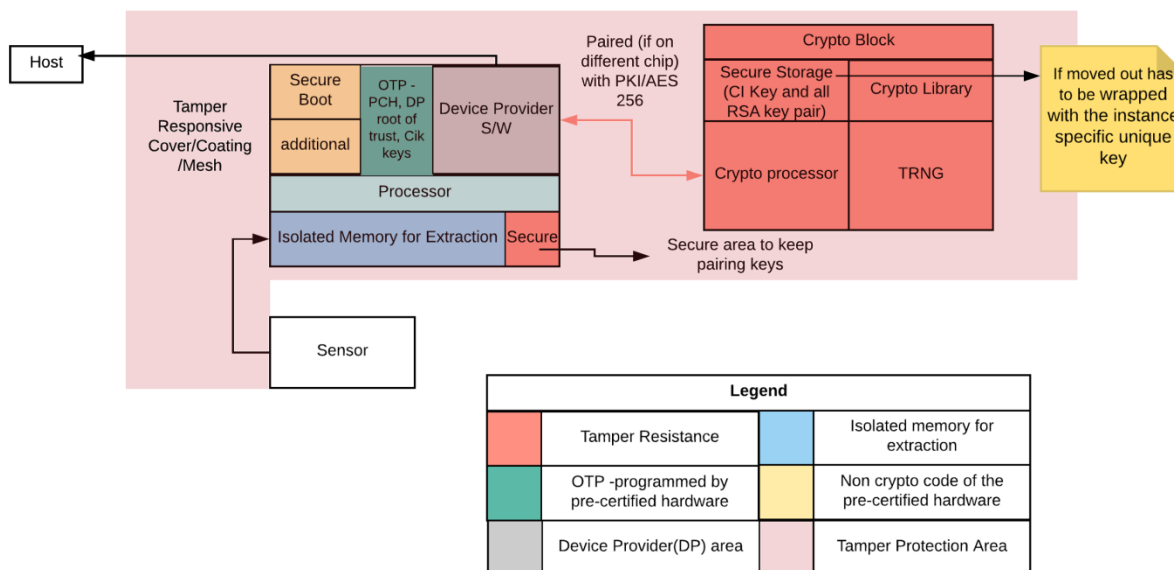
Reference design for L1 with System Level Tamper
